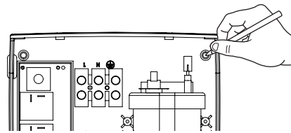
Mark the mounting holes
